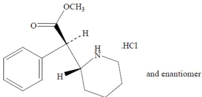
Figure 2: Structural Formula – methylphenidate hydrochloride
